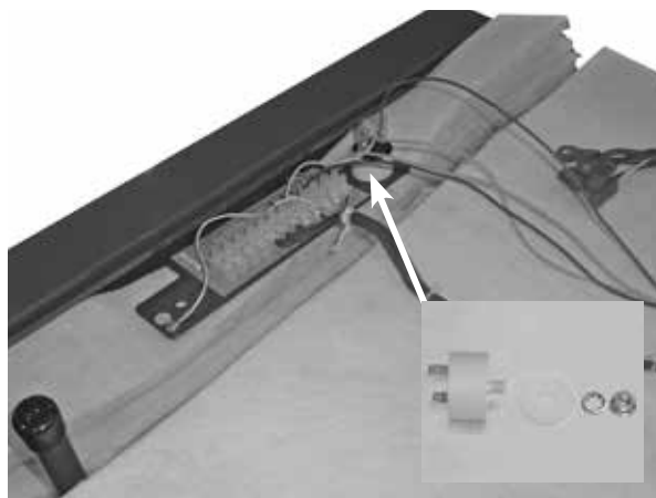
Capacitator for exhaust fan - 1 \mu F
